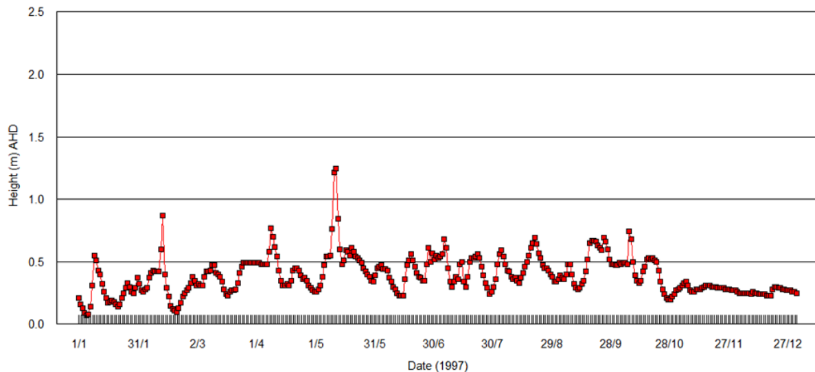
Figure 2. Water level changes in a coastal lagoon with an entrance open to coastal waters.
