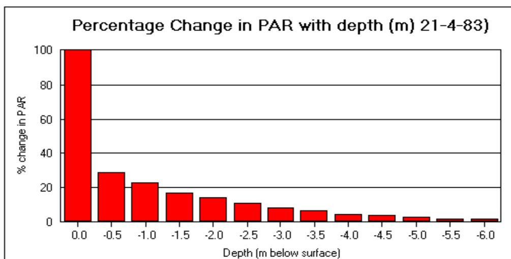
Figure 4. Actual percentage changes in PAR at Station 1 - Wyee Point on the morning of 21-4-83.
