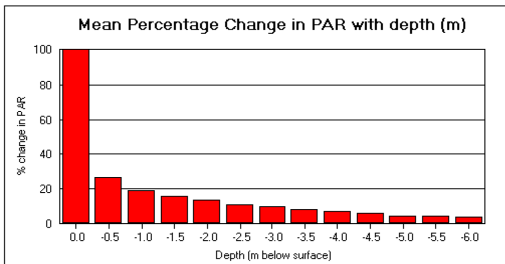
Figure 3. Mean percentage changes in PAR with depth at Station 1 - Wyee Point over 12 months.
